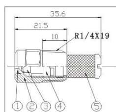
1.Orifice 2.Body 3.Cyclone Core 4.Plug 5.strainer mesh
